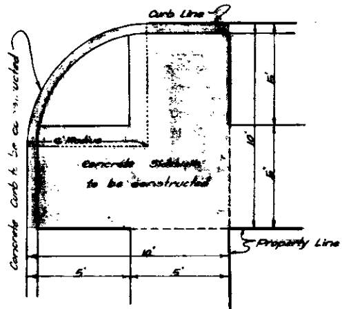
PLAN OF RETURN Scale 1" = 3'
